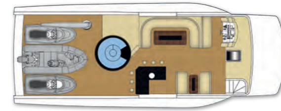
FLY-BRIDGE
