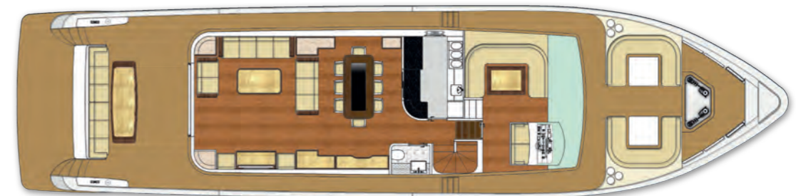
MAIN DECK
